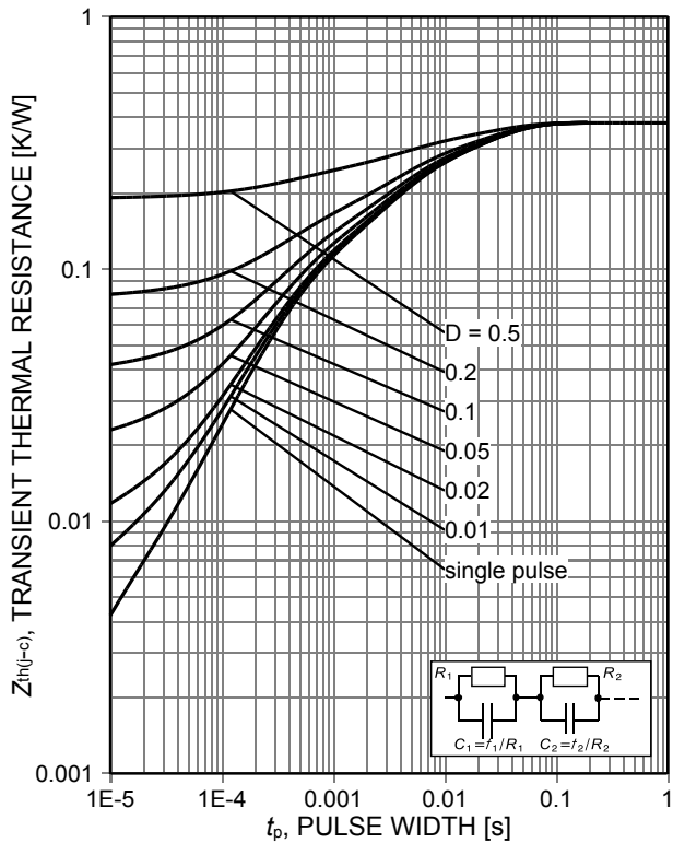
Figure 19. IGBT transient thermal resistance ( D=t_p/T )
