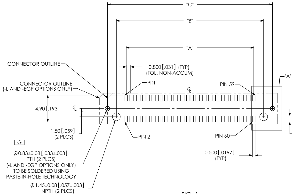
FIG. 1 ALL OPTIONS EXCEPT - EGPS (-030 POSITION SHOWN) (ALL DIMENSIONS ARE SYMMETRIC ABOUT THE CENTERLINE)
