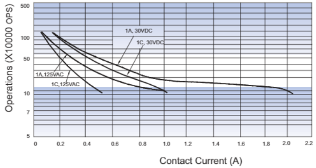
ENDURANCE CURVE
