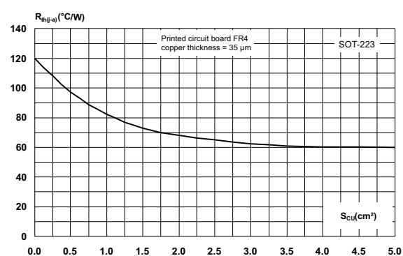
Figure 15. Thermal resistance junction to ambient versus copper surface under tab (SOT-223)
