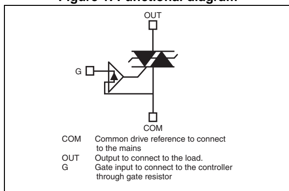
Figure 1. Functional diagram
