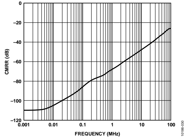
Figure 35. CMRR vs. Frequency
