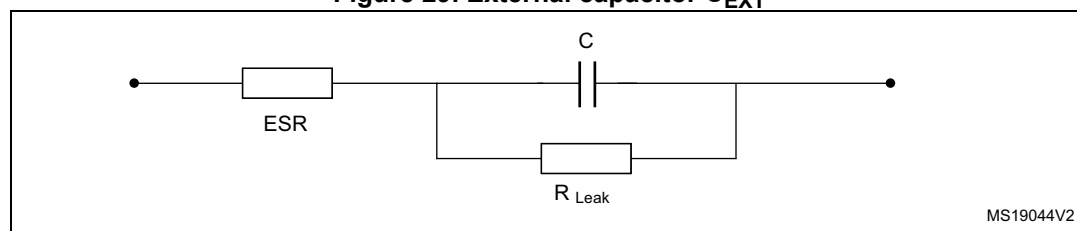
Figure 29. External capacitor C_{EXT}
