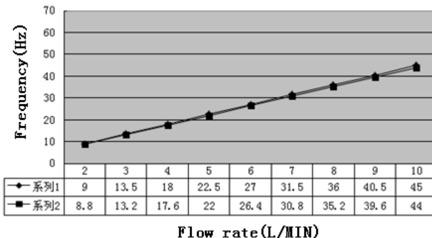
Flow rate vs. frequency plot
