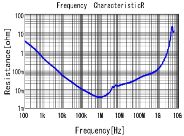
■ GRT31CR61H106KE01 R DCOV, 25degC
