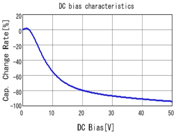
■ GRT31CR61H106KE01 C-DC bias capchange, 25.0degC, AC1.
