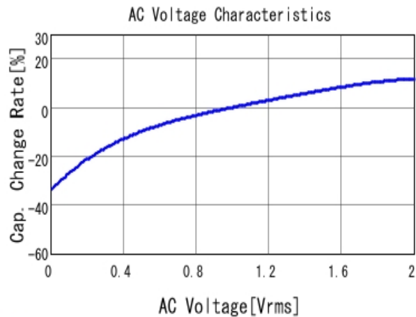
■ GRT31CR61H106KE01 C-AC Voltage capchange, DCOV, 25.0d
