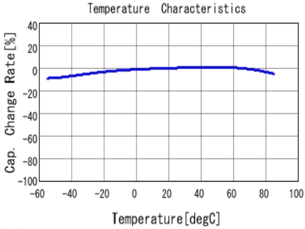
■ GRT31CR61H106KE01 C-Temp. capchange, DC0.0V, AC1.0V rm
