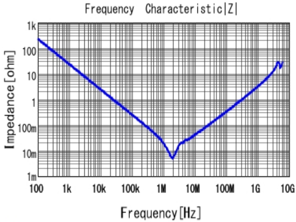
■ GRT31CR61H106KE01 |Z| DCOV, 25degC
