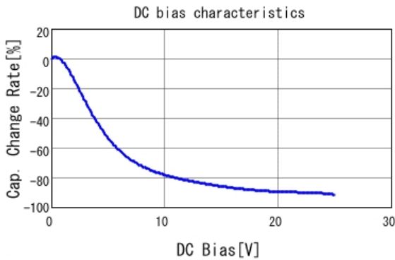
■ GRT21BR61E226ME13 C-DC bias capchange, 25.0degC, AC0.
