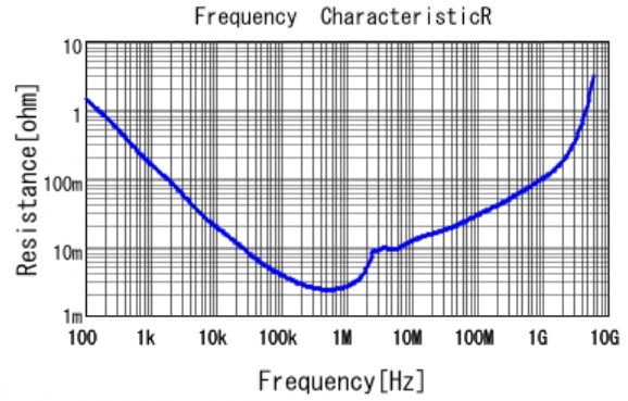
■ GRT21BR61E226ME13 R DCOV, 25degC
