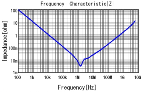
■ GRT21BR61E226ME13 |Z| DCOV, 25degC
