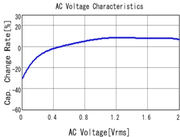
■ GRT21BR61A226ME13 C-AC Voltage capchange, DCOV, 25.0d
