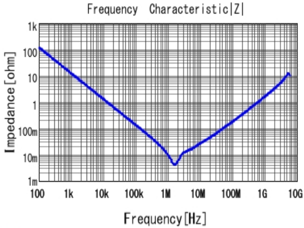
■ GRT21BR61A226ME13 |Z| DCOV, 25degC
