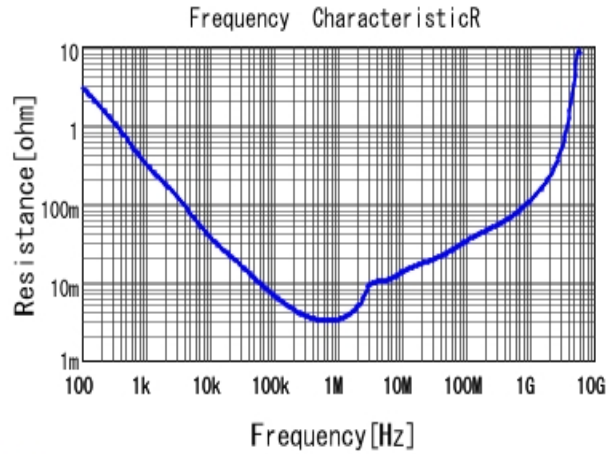
■ GRT21BR61A226ME13 R DCOV, 25degC
