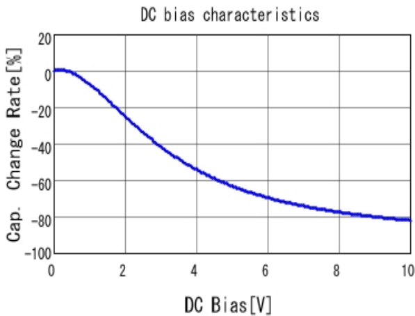
■ GRT21BR61A226ME13 C-DC bias capchange, 25.0degC, AC0.
