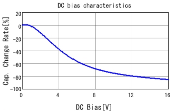
■ GRT188C81C475KE13 C-DC bias capchange, 25.0degC, AC1V
