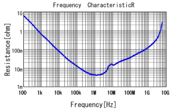
■ GRT188C81C475KE13 R DCOV, 25degC
