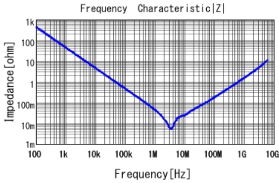
■ GRT188C81C475KE13 |Z| DCOV, 25degC
