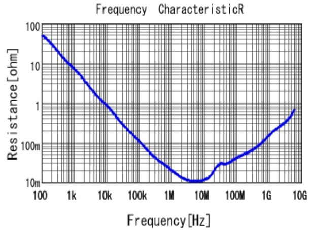
■ GRT155R70J105KE01 R DCOV, 25degC
