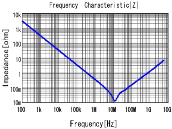
■ GRT155R70J105KE01 |Z| DCOV, 25degC
