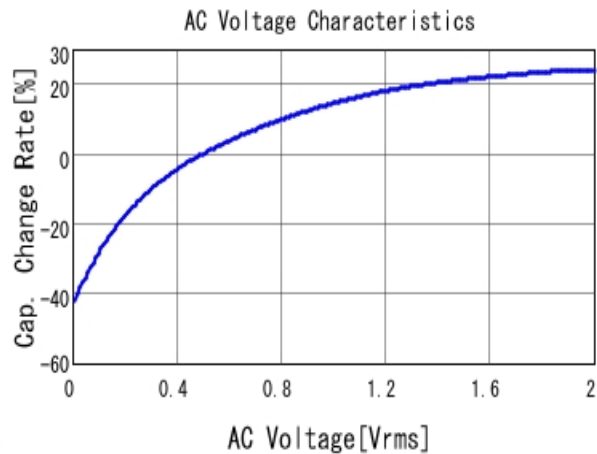
■ GRT155R70J105KE01 C-AC Voltage capchange, DCOV, 25.0d
