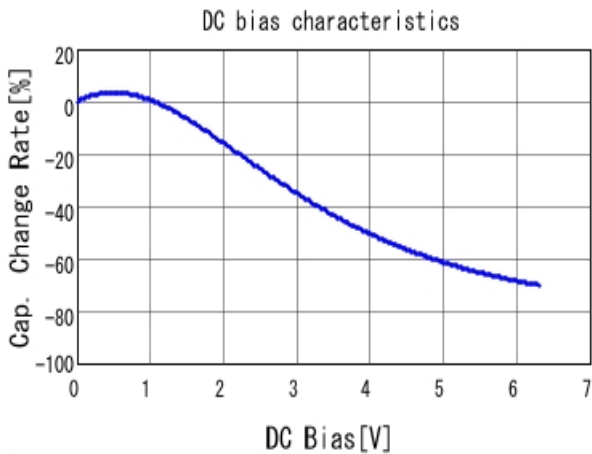
■ GRT155R70J105KE01 C-DC bias capchange, 25.0degC, AC0.
