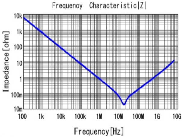
■ GRT155R6YA474KE01 |Z| DCOV, 25degC
