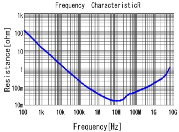
■ GRT155R6YA474KE01 R DCOV, 25degC
