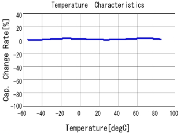
■ GRT155R6YA474KE01 C-Temp. capchange, DC0.0V, AC1.0V rm
