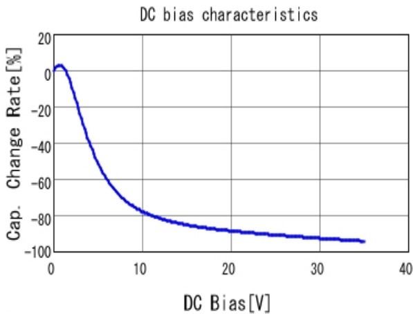
■ GRT155R6YA474KE01 C-DC bias capchange, 25.0degC, AC1.
