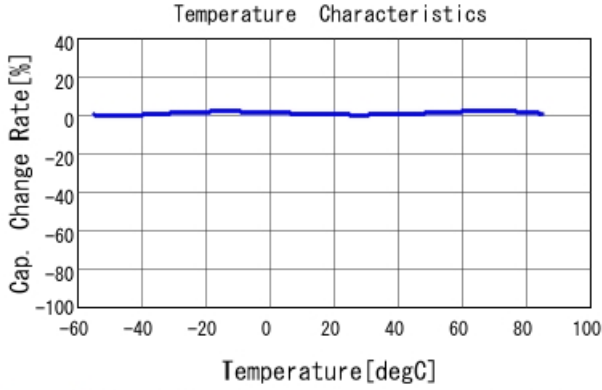
GRT155R61E474KE01 C-Temp. capchange, DC0.0V, AC1.C
