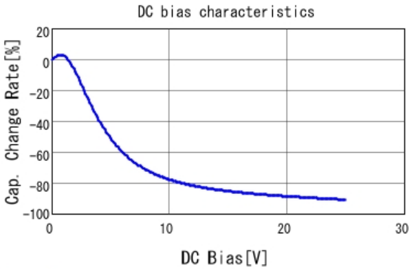
GRT155R61E474KE01 C-DC bias capchange, 25.0degC, A
