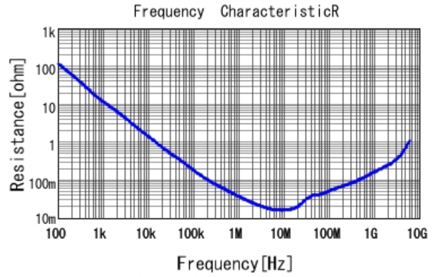
GRT155R61E474KE01 R DCOV, 25degC
