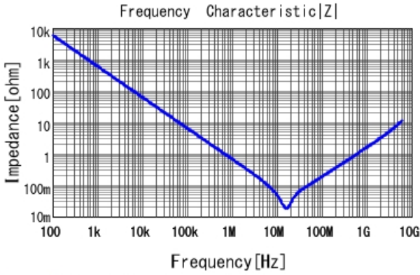
GRT155R61E474KE01 |Z| DCOV, 25degC
