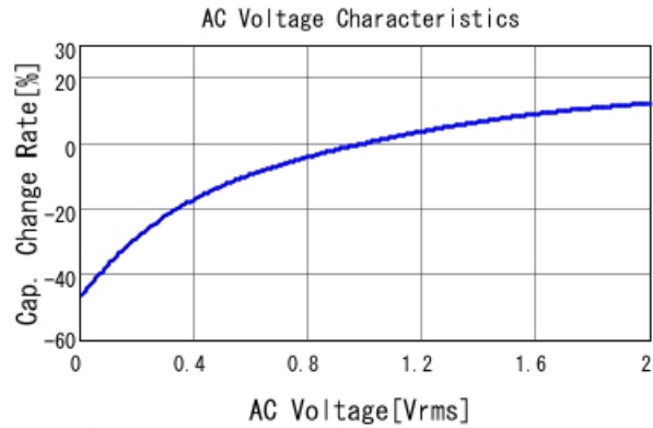
GRT155R61E474KE01 C-AC Voltage capchange, DCOV, 25
