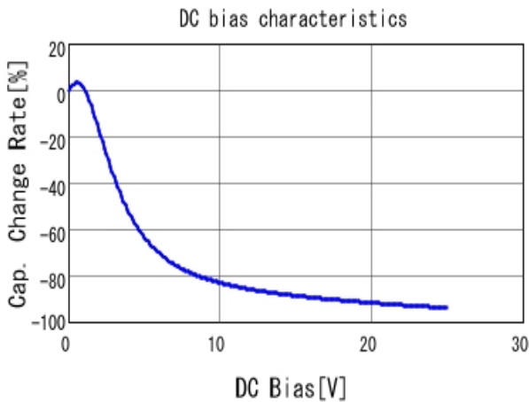
■ GRT155R61E105KE01 C-DC bias capchange, 25.0degC, AC1.
