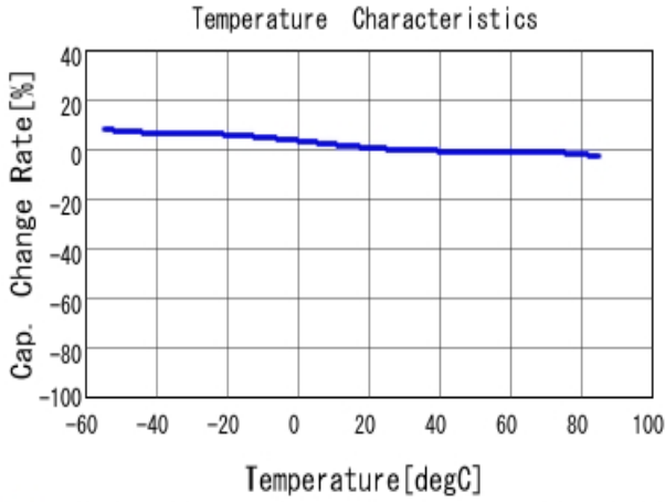
■ GRT155R61E105KE01 C-Temp. capchange, DC0.0V, AC1.0V rm
