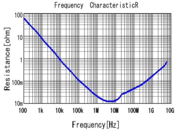
■ GRT155R61E105KE01 R DCOV, 25degC
