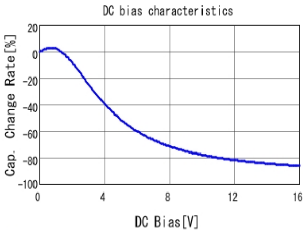
■ GRT155R61C474KE01 C-DC bias capchange, 25.0degC, AC1.
