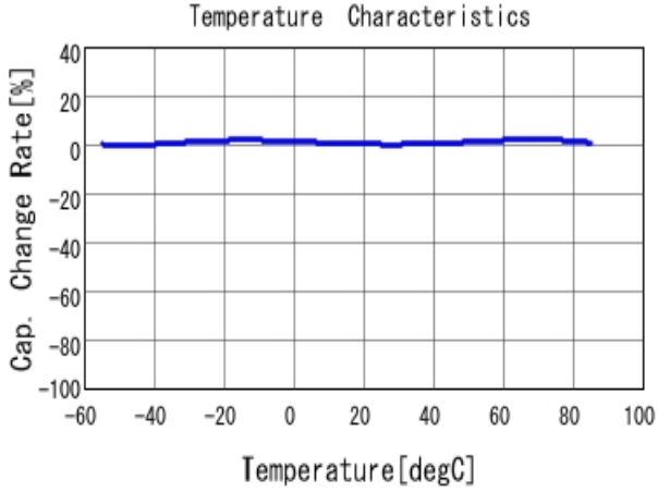
GRT155R61C474KE01 C-Temp. capchange, DC0.0V, AC1.0V r m
