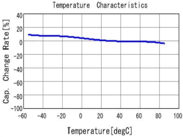
■ GRT155R61C105KE01 C-Temp. capchange, DC0.0V, AC1.0V rm
