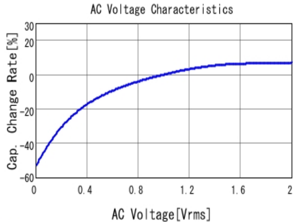
GRT155R61C105KE01 C-AC Voltage capchange, DCOV, 25.0d
