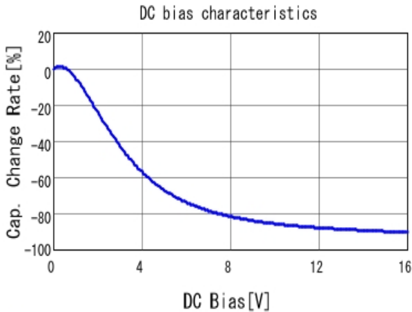
GRT155R61C105KE01 C-DC bias capchange, 25.0degC, AC1.
