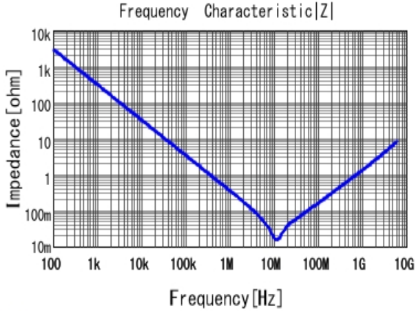
GRT155R61C105KE01 |Z| DCOV, 25degC
