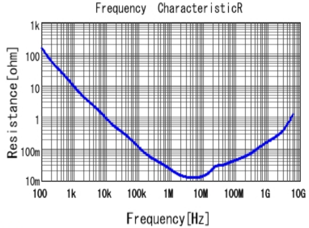
GRT155R61C105KE01 R DCOV, 25degC
