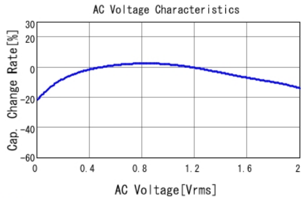
GRT155R60J475ME13 C-AC Voltage capchange, DCOV, 25.0d
