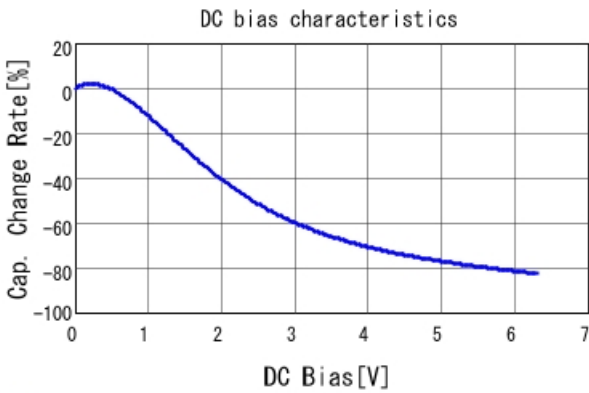
GRT155R60J475ME13 C-DC bias capchange, 25.0degC, AC0.
