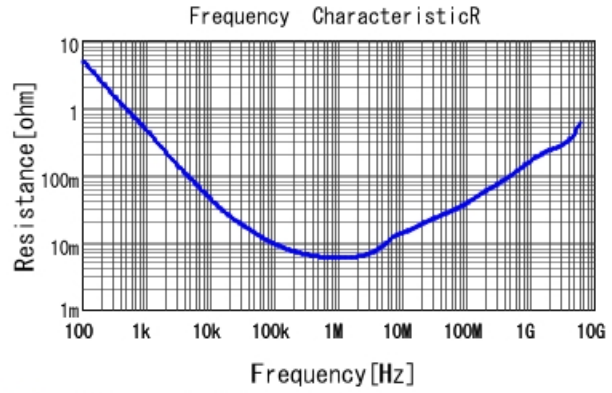
GRT155R60J475ME13 R DCOV, 25degC
