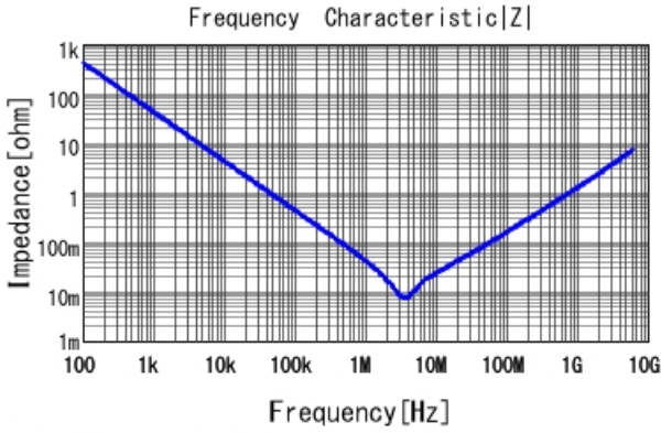
GRT155R60J475ME13 |Z| DCOV, 25degC
