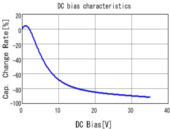
■ GRT155C8YA224KE01 C-DC bias capchange, 25.0degC, AC1.
