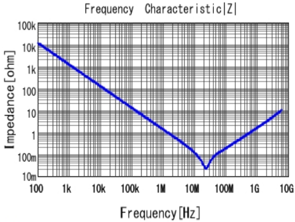
■ GRT155C8YA224KE01 |Z| DCOV, 25degC
