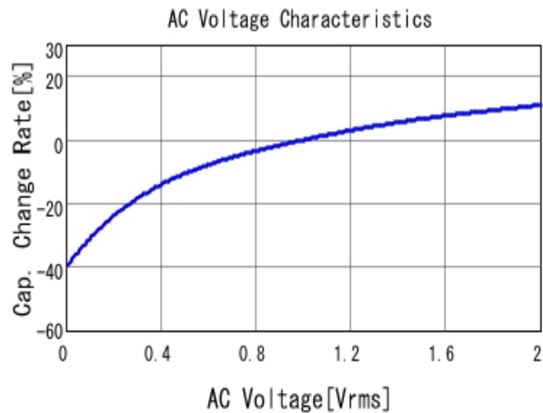
■ GRT155C8YA224KE01 C-AC Voltage capchange, DCOV, 25.0d
