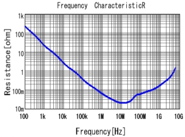
■ GRT155C8YA224KE01 R DCOV, 25degC
