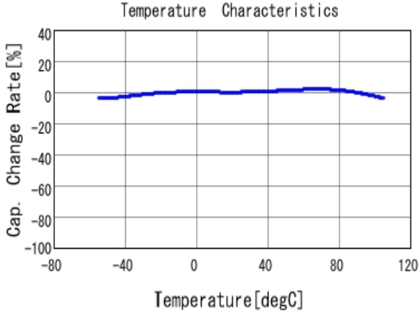
GRT155C8YA224KE01 C-Temp. capchange, DC0.0V, AC1.0V rm
