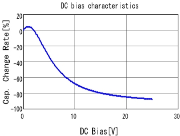
■ GRT155C81E224KE01 C-DC bias capchange, 25.0degC, AC1.
