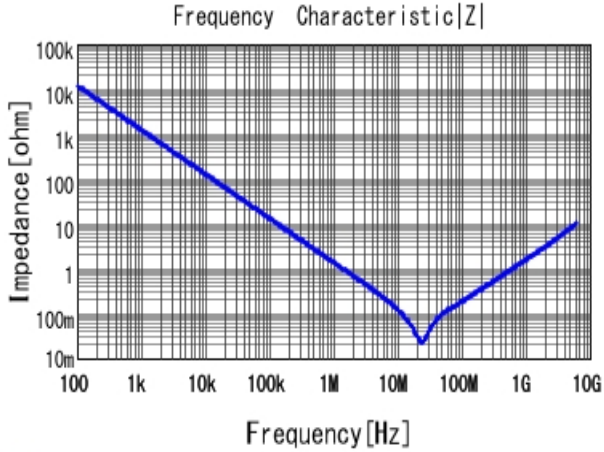
■ GRT155C81E224KE01 |Z| DCOV, 25degC
