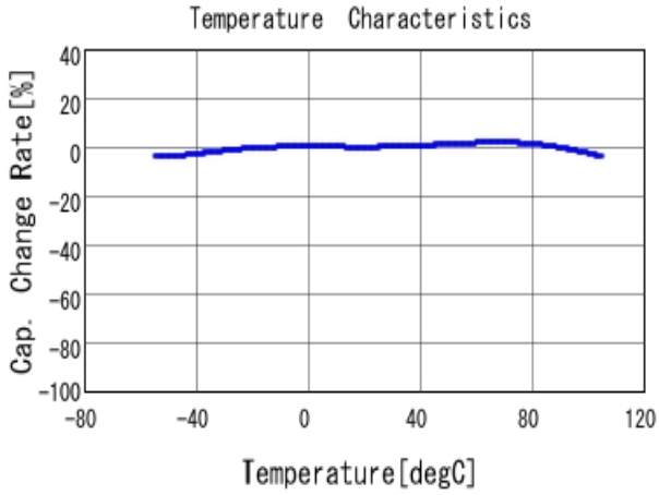
GRT155C81E224KE01 C-Temp. capchange, DC0.0V, AC1.0V r m
