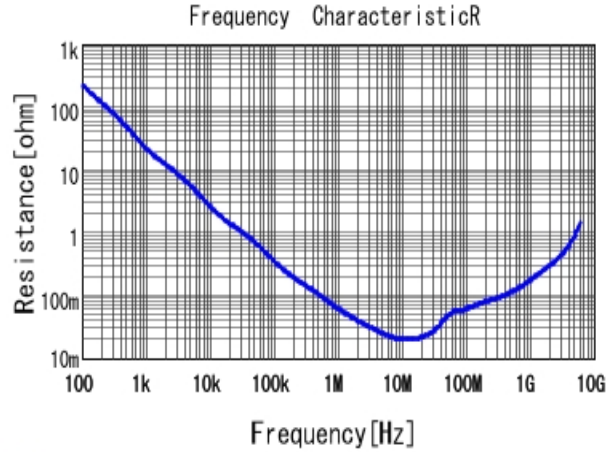
■ GRT155C81E224KE01 R DCOV, 25degC
