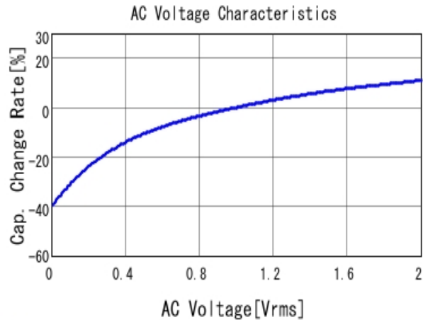
■ GRT155C81E224KE01 C-AC Voltage capchange, DCOV, 25.0d
