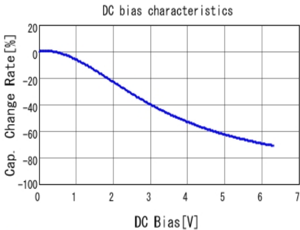
■ GRT033C80J224KE01 C-DC bias capchange, 25.0degC, AC0.
