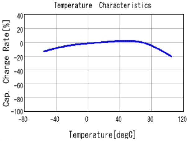
■ GRT033C80J224KE01 C-Temp. capchange, DC0.0V, AC0.1V r m
