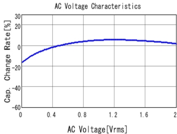
■ GRT033C80J224KE01 C-AC Voltage capchange, DCOV, 25.0d
