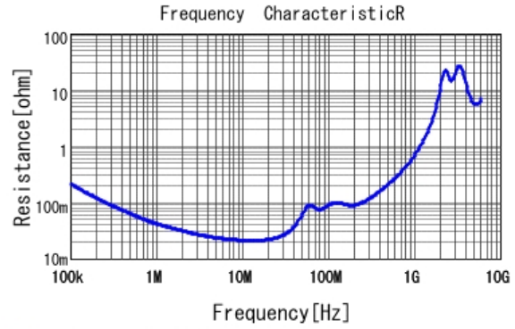
■ GRM55DR73A683KW01 R DCOV, 25degC
