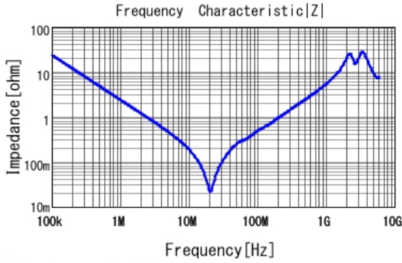
■ GRM55DR73A683KW01 |Z| DCOV, 25degC
