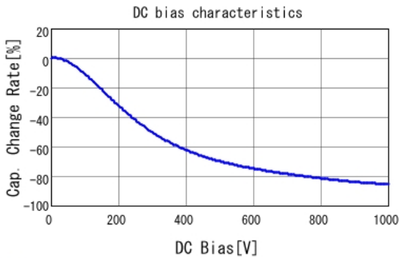
■ GRM55DR73A683KW01 C-DC bias capchange, 25.0degC, AC1V
