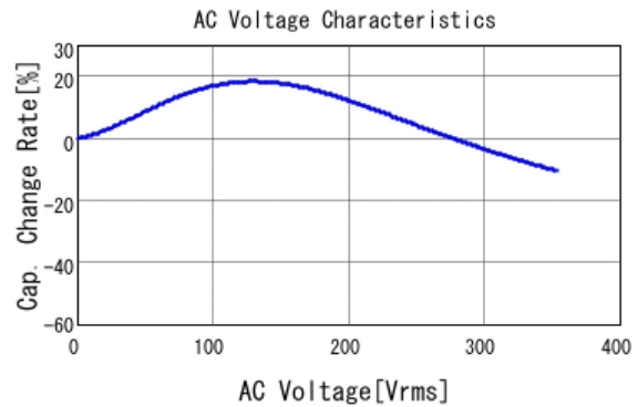
■ GRM55DR73A683KW01 C-AC Voltage capchange, DCOV, 25.0d
