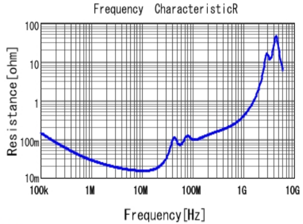
■ GRM55DR73A104KW01 R DCOV, 25degC
