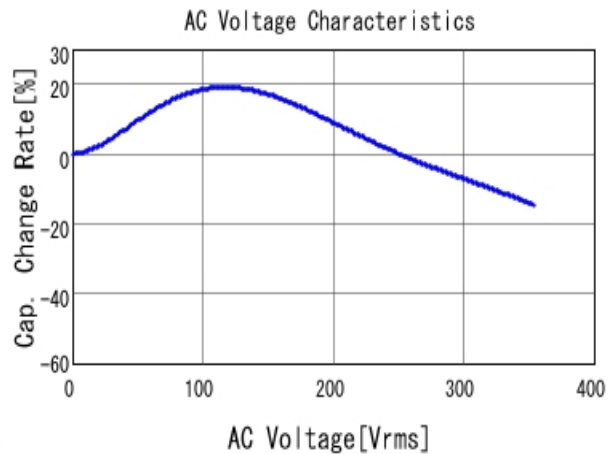
■ GRM55DR73A104KW01 C-AC Voltage capchange, DCOV, 25.0d
