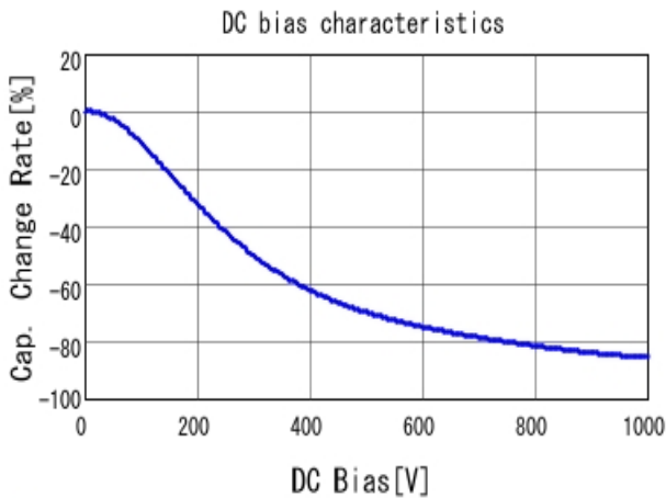
■ GRM55DR73A104KW01 C-DC bias capchange, 25.0degC, AC1V
