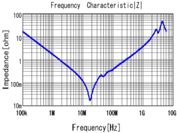
■ GRM55DR73A104KW01 |Z| DCOV, 25degC
