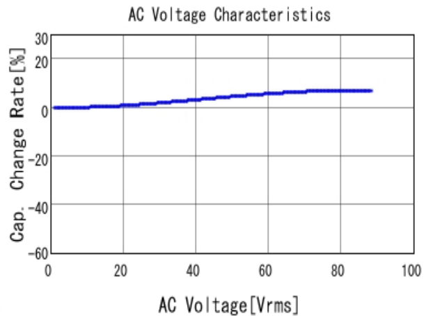
■ GRM55DR72E334KW01 C-AC Voltage capchange, DCOV, 25.0d
