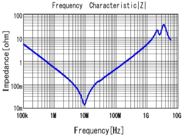
■ GRM55DR72E334KW01 |Z| DCOV, 25degC
