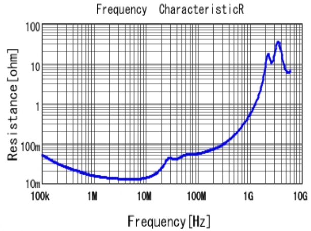
■ GRM55DR72E334KW01 R DCOV, 25degC
