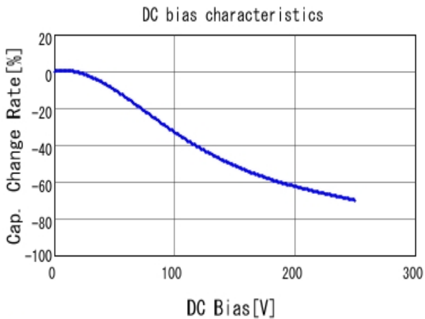
■ GRM55DR72E334KW01 C-DC bias capchange, 25.0degC, AC1V
