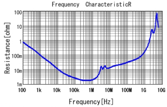
■ GRM55DR61H106KA88 R DCOV, 25degC
