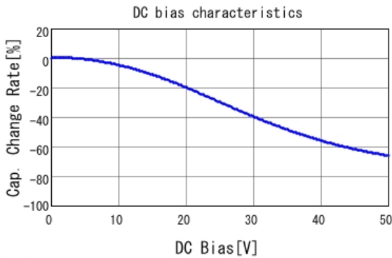
■ GRM55DR61H106KA88 C-DC bias capchange, 25.0degC, AC1.
