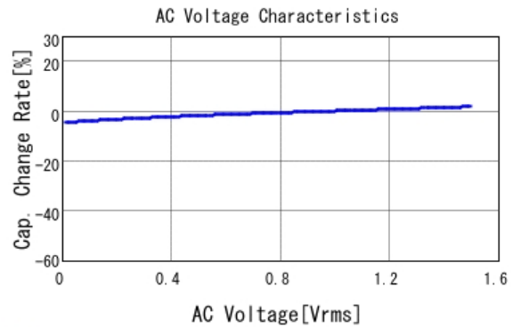
■ GRM55DR61H106KA88 C-AC Voltage capchange, DCOV, 25.0d
