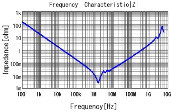
■ GRM55DR61H106KA88 |Z| DCOV, 25degC
