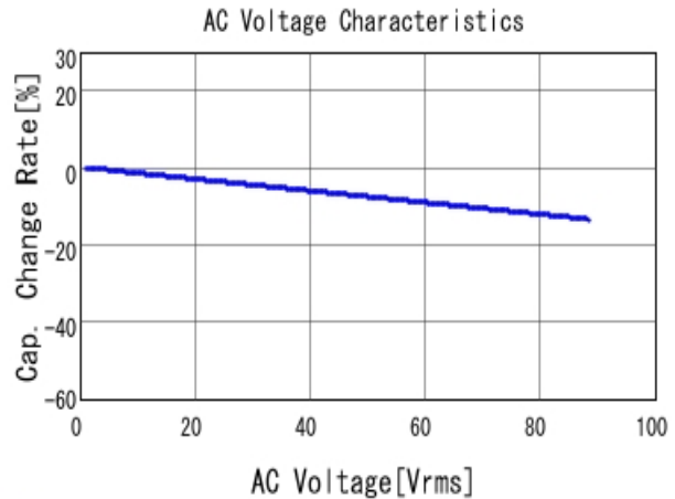
■ GRM43QR72E154KW01 C-AC Voltage capchange, DCOV, 25.0d
