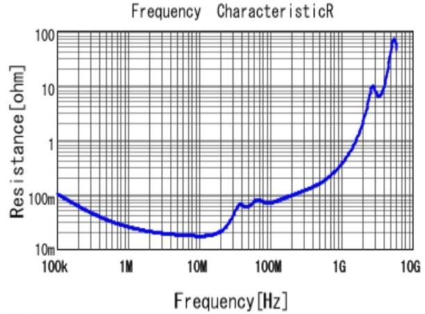
■ GRM43QR72E154KW01 R DCOV, 25degC
