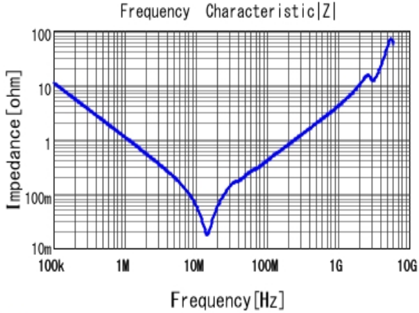
■ GRM43QR72E154KW01 |Z| DCOV, 25degC
