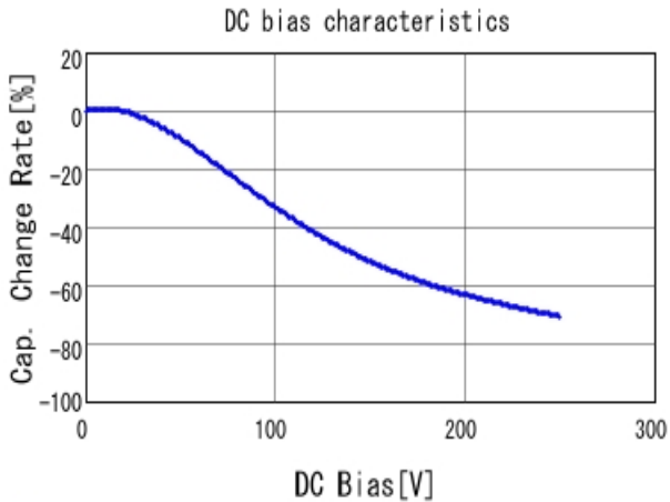
■ GRM43QR72E154KW01 C-DC bias capchange, 25.0degC, AC1V
