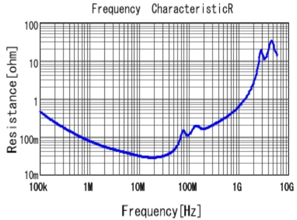
■ GRM43DR73A333KW01 R DCOV, 25degC
