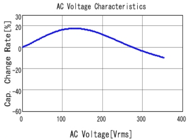
■ GRM43DR73A333KW01 C-AC Voltage capchange, DCOV, 25.0d
