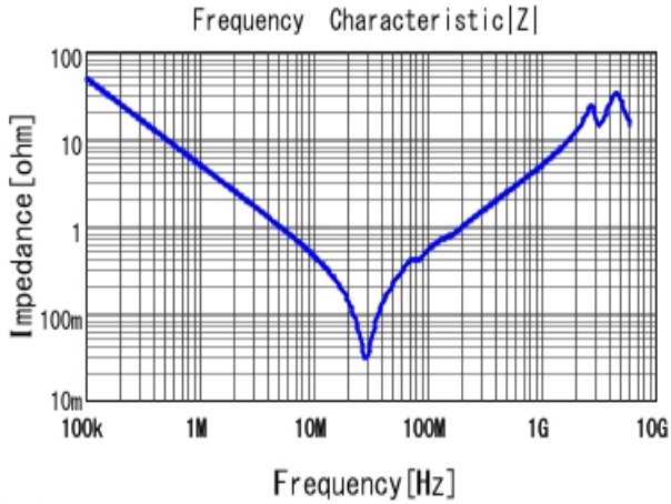
■ GRM43DR73A333KW01 |Z| DCOV, 25degC
