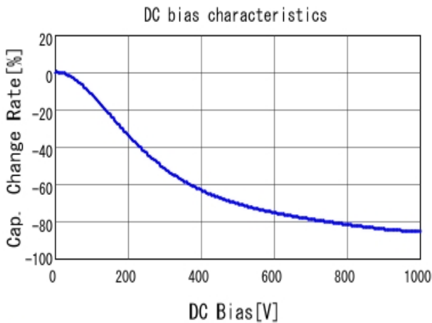
■ GRM43DR73A333KW01 C-DC bias capchange, 25.0degC, AC1V
