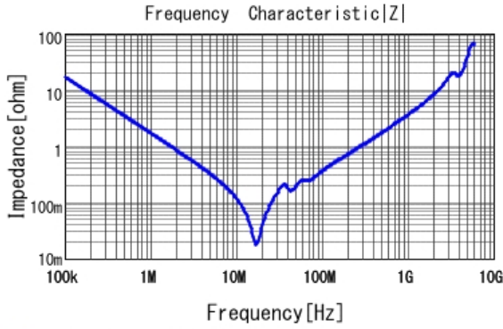
■ GRM43DR72J104KW01 |Z| DC0V, 25degC
