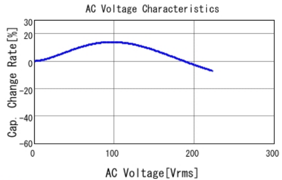
■ GRM43DR72J104KW01 C-AC Voltage capchange, DC0V, 25.0d
