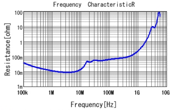
■ GRM43DR72E474KW01 R DCOV, 25degC
