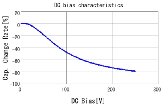
■ GRM43DR72E474KW01 C-DC bias capchange, 25.0degC, AC1V
