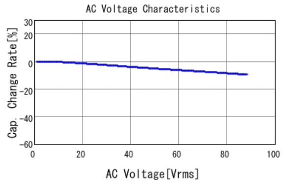
■ GRM43DR72E474KW01 C-AC Voltage capchange, DCOV, 25.0d
