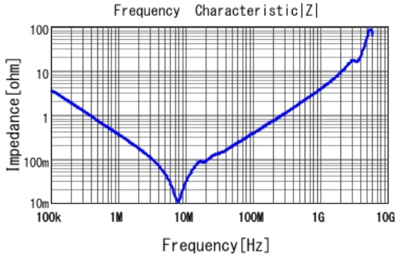
■ GRM43DR72E474KW01 |Z| DCOV, 25degC
