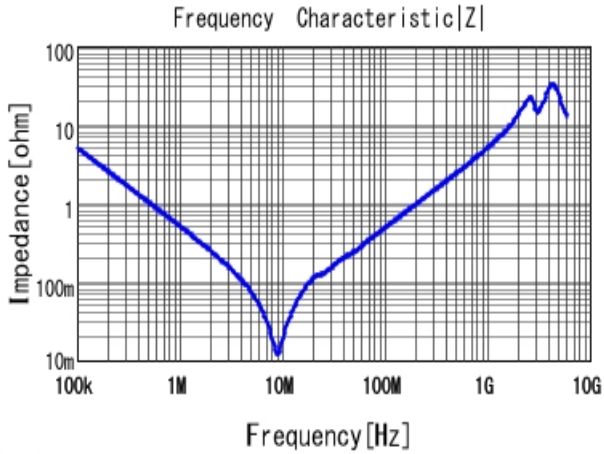
■ GRM43DR72E334KW01 |Z| DCOV, 25degC
