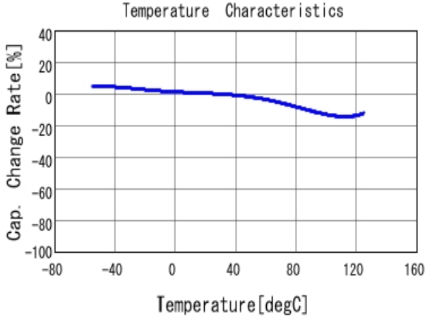
■ GRM43DR72E334KW01 C-Temp. capchange, DCOV, AC1Vrms
