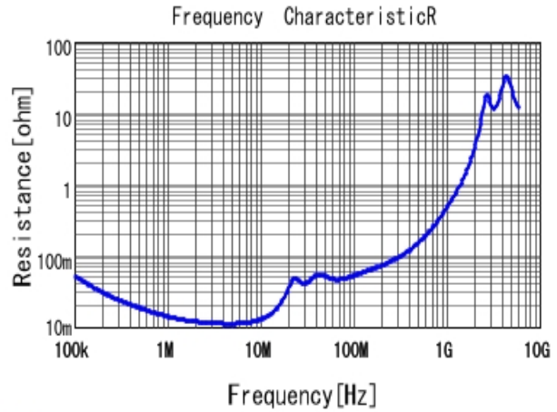
■ GRM43DR72E334KW01 R DCOV, 25degC
