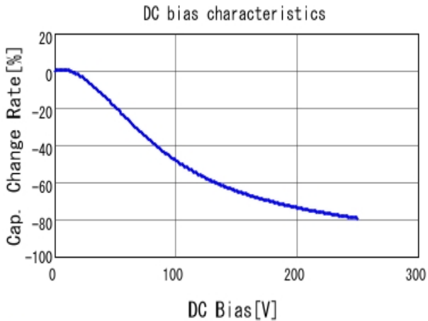
■ GRM43DR72E334KW01 C-DC bias capchange, 25.0degC, AC1V
