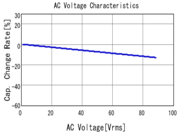
■ GRM43DR72E334KW01 C-AC Voltage capchange, DCOV, 25.0d
