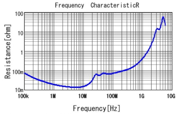
■ GRM43DR72E224KW01 R DCOV, 25degC
