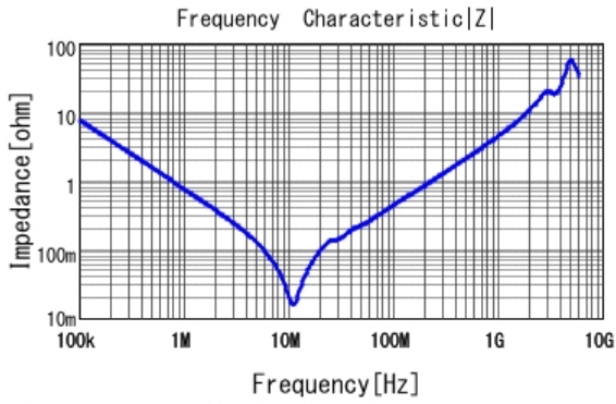
■ GRM43DR72E224KW01 |Z| DCOV, 25degC
