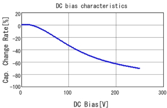
■ GRM43DR72E224KW01 C-DC bias capchange, 25.0degC, AC1V
