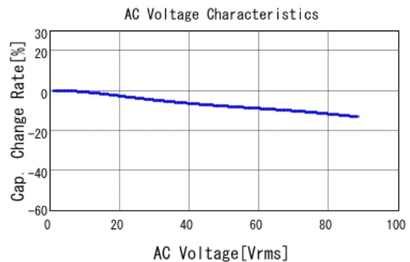
■ GRM43DR72E224KW01 C-AC Voltage capchange, DCOV, 25.0d
