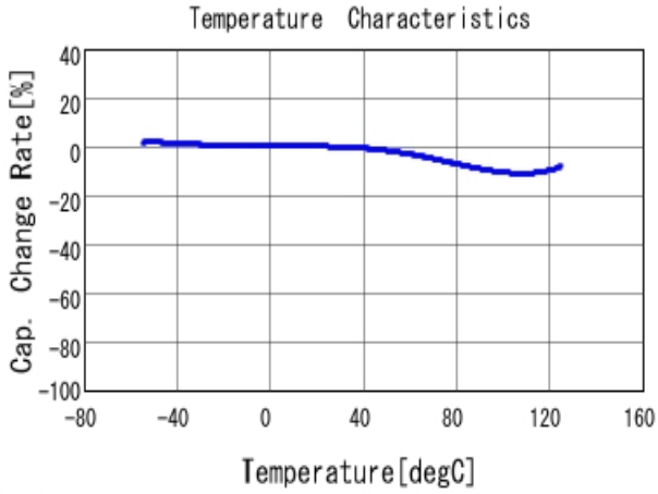
■ GRM32RR71H105KA01 C-Temp. capchange, DC0.0V, AC1.0V rm
