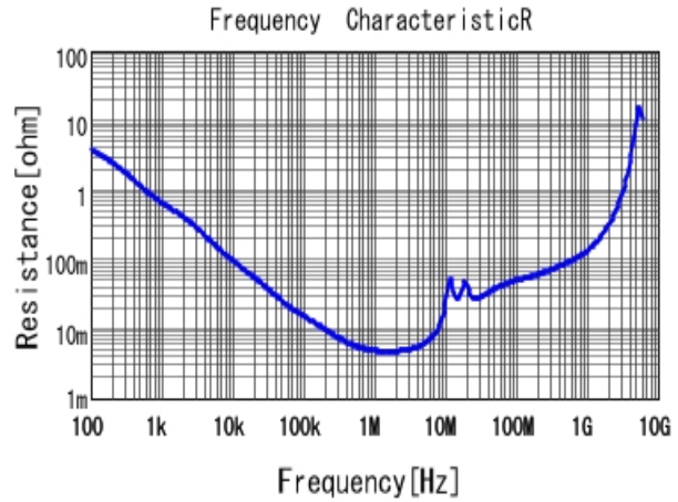
■ GRM32RR71H105KA01 R DCOV, 25degC
