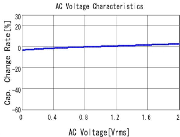
■ GRM32RR71H105KA01 C-AC Voltage capchange, DCOV, 25.0d
