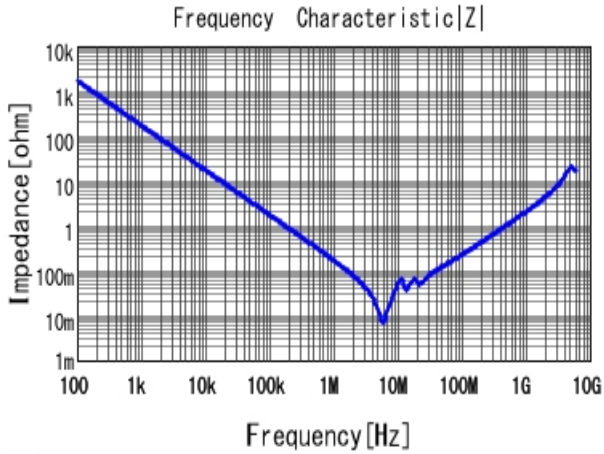
■ GRM32RR71H105KA01 |Z| DCOV, 25degC
