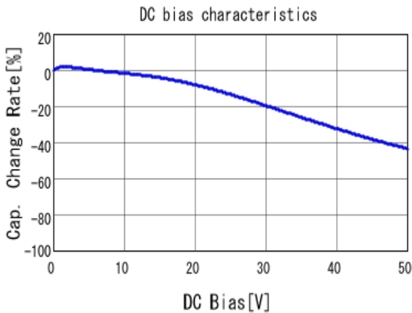
■ GRM32RR71H105KA01 C-DC bias capchange, 25.0degC, AC1.
