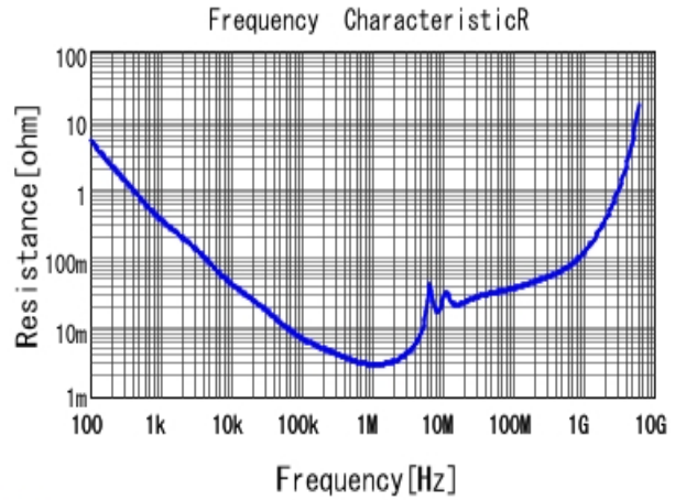
■ GRM32ER72A225KA35 R DCOV, 25degC
