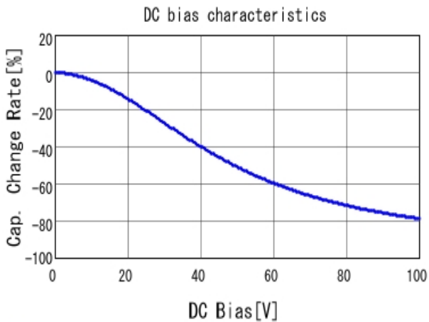
■ GRM32ER72A225KA35 C-DC bias capchange, 25.0degC, AC1.
