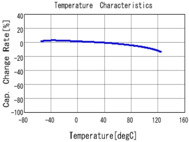
■ GRM32ER72A225KA35 C-Temp. capchange, DC0.0V, AC1.0V r m
