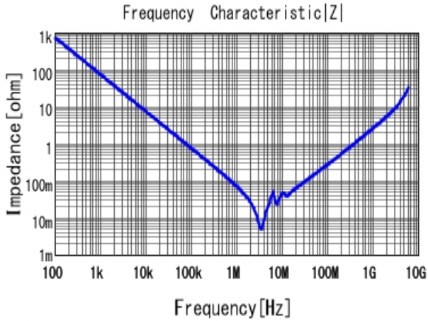
■ GRM32ER72A225KA35 |Z| DCOV, 25degC
