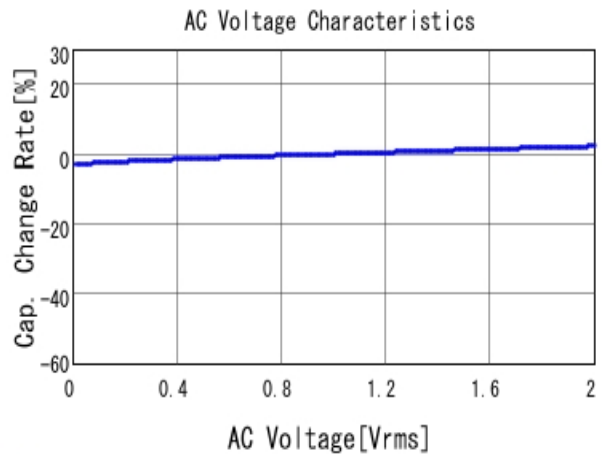
■ GRM32ER72A225KA35 C-AC Voltage capchange, DCOV, 25.0d
