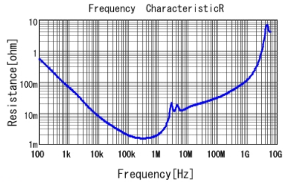
■ GRM32ER71J106KA12 R DCOV, 25degC
