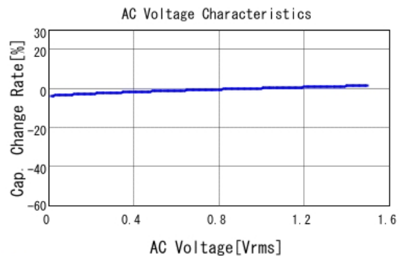
■ GRM32ER71J106KA12 C-AC Voltage capchange, DCOV, 25.0d
