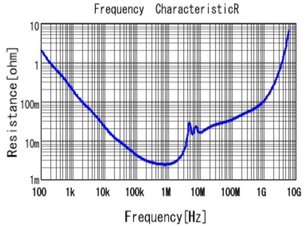
■ GRM32ER71H475KA88 R DCOV, 25degC
