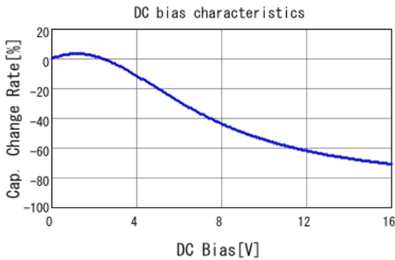
■ GRM32ER71C226MEA8 C-DC bias capchange, 25.0degC, AC0.
