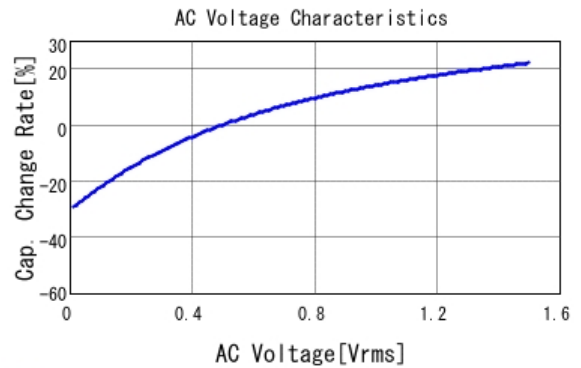
■ GRM32ER71C226MEA8 C-AC Voltage capchange, DCOV, 25.0d
