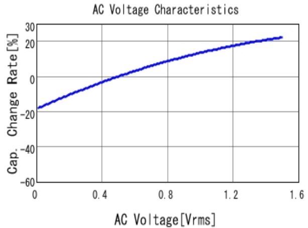
■ GRM32ER61E226KE15 C-AC Voltage capchange, DCOV, 25.0d
