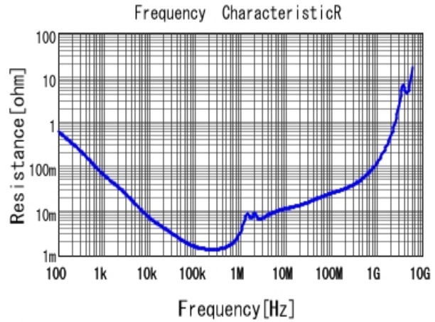
■ GRM32ER61C476KE15 R DCOV, 25degC
