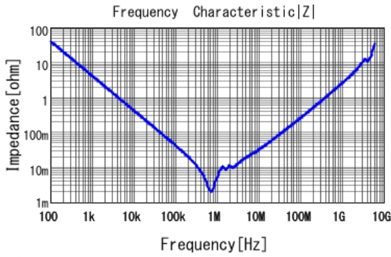
■ GRM32ER60J476ME20 |Z| DCOV, 25degC
