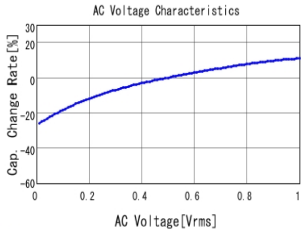
■ GRM32ER60J107ME20 C-AC Voltage capchange, DCOV, 25.0d
