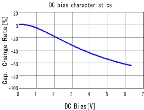
■ GRM32ER60J107ME20 C-DC bias capchange, 25.0degC, AC0.
