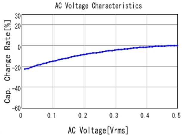
■ GRM32ER60G337ME05 C-AC Voltage capchange, DCOV, 25.0d
