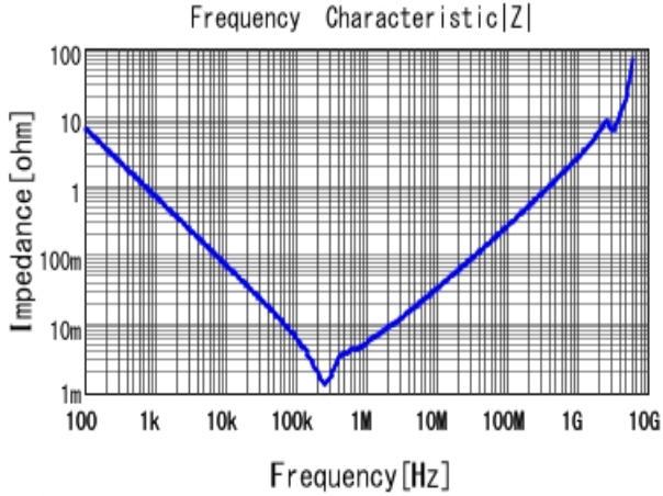
■ GRM32ER60G337ME05 |Z| DCOV, 25degC
