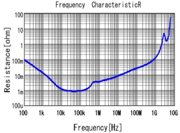
■ GRM32ER60G337ME05 R DCOV, 25degC
