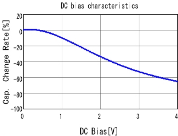
■ GRM32ER60G337ME05 C-DC bias capchange, 25.0degC, AC0.
