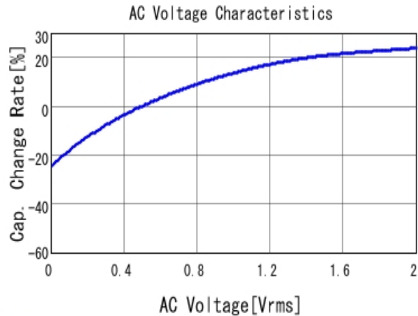
■ GRM32EC81C476KE15 C-AC Voltage capchange, DCOV, 25.0d
