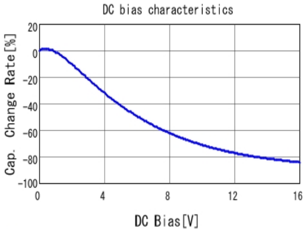
■ GRM32EC81C476KE15 C-DC bias capchange, 25.0degC, AC0.
