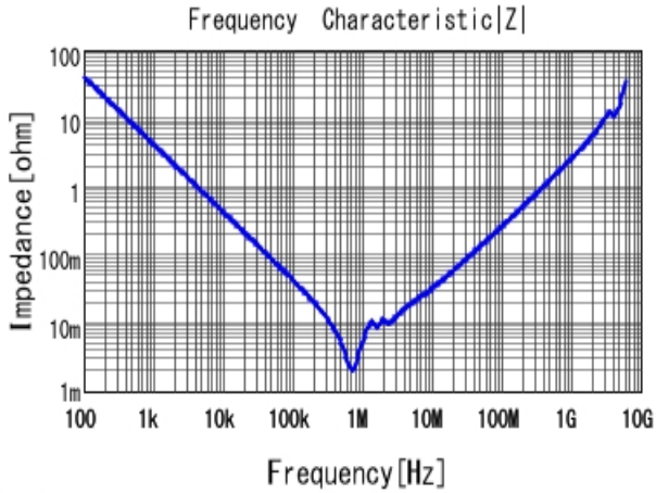
■ GRM32EC81C476KE15 |Z| DCOV, 25degC
