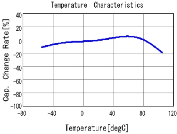
■ GRM32EC81C476KE15 C-Temp. capchange, DC0.0V, AC0.5V rm
