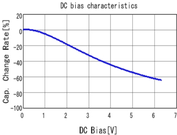
■ GRM32EC80J107ME20 C-DC bias capchange, 25.0degC, AC0.
