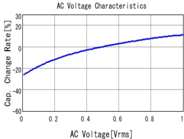
■ GRM32EC80J107ME20 C-AC Voltage capchange, DCOV, 25.0d
