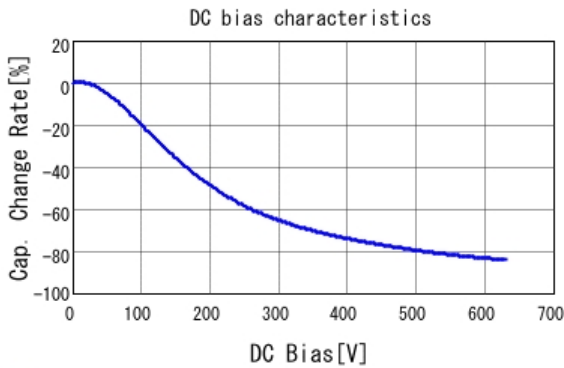
■ GRM32DR72J333KW01 C-DC bias capchange, 25.0degC, AC1V
