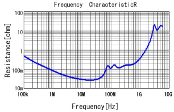
■ GRM32DR72J333KW01 R DCOV, 25degC
