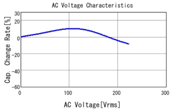
■ GRM32DR72J333KW01 C-AC Voltage capchange, DCOV, 25.0d
