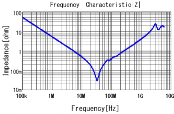
■ GRM32DR72J333KW01 |Z| DCOV, 25degC
