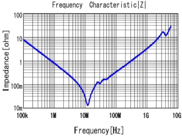
■ GRM32DR72E224KW01 |Z| DCOV, 25degC
