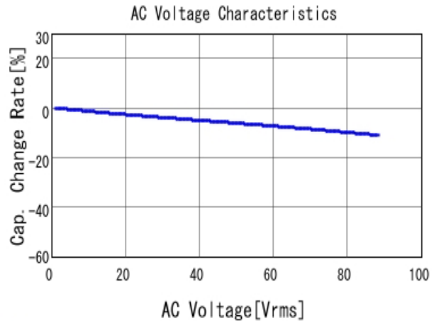
■ GRM32DR72E224KW01 C-AC Voltage capchange, DCOV, 25.0d
