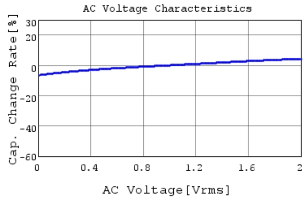
GRM32DR61E106KA12 C-AC Voltage capchange, Dc
