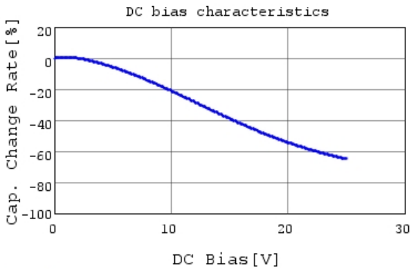
GRM32DR61E106KA12 C-DC bias capchange, 25.0c
