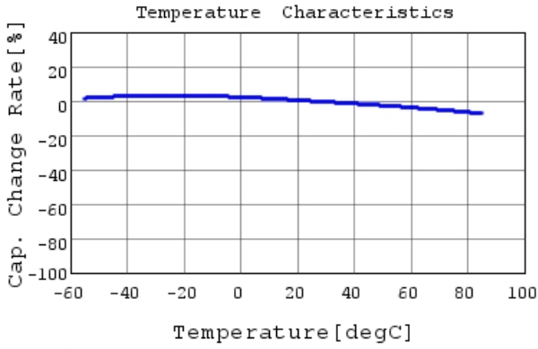
GRM32DR61E106KA12 C-Temp. capchange, DC0.0V,
