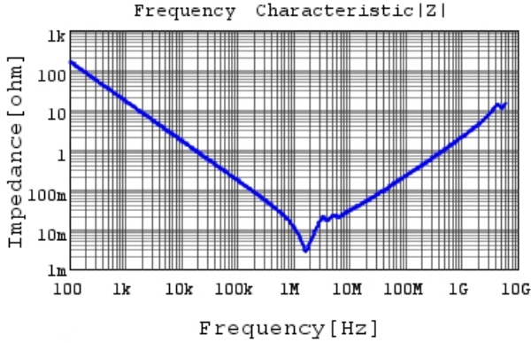
GRM32DR61E106KA12 |Z| DCOV, 25degC
