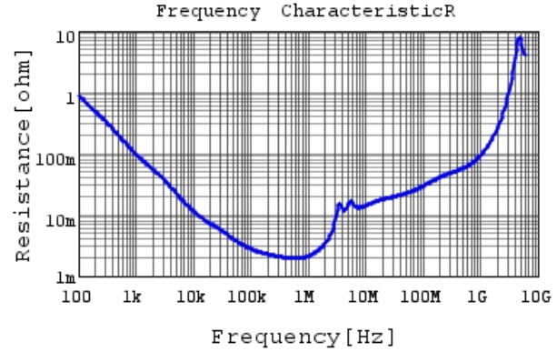
GRM32DR61E106KA12 R DCOV, 25degC
