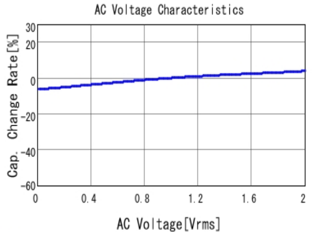
■ GRM32DC72A475KE01 C-AC Voltage capchange, DCOV, 25.0d
