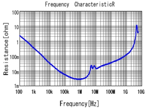
■ GRM32DC72A475KE01 R DCOV, 25degC
