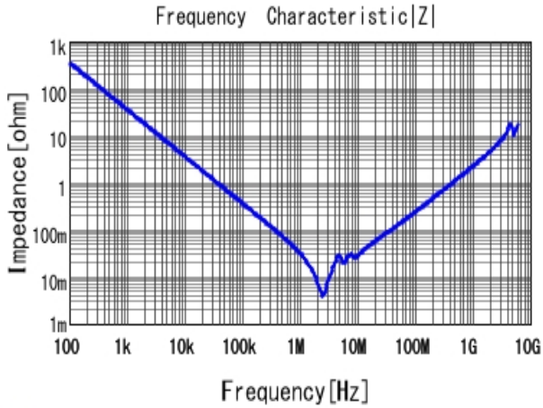
■ GRM32DC72A475KE01 |Z| DCOV, 25degC
