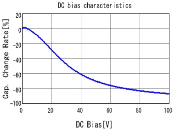
■ GRM32DC72A475KE01 C-DC bias capchange, 25.0degC, AC1.
