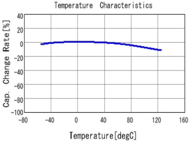
■ GRM32DC72A475KE01 C-Temp. capchange, DC0.0V, AC1.0V rm
