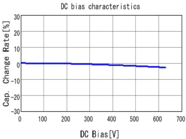
■ GRM32D7U2J103JW31 C-DC bias capchange, 25.0degC, AC1V
