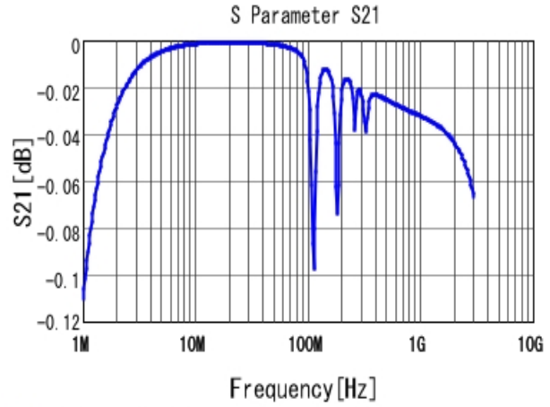
■ GRM32D7U2J103JW31 S21 DCOV, 25degC
