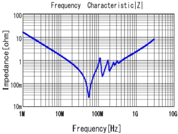
■ GRM32D7U2J103JW31 |Z| DCOV, 25degC
