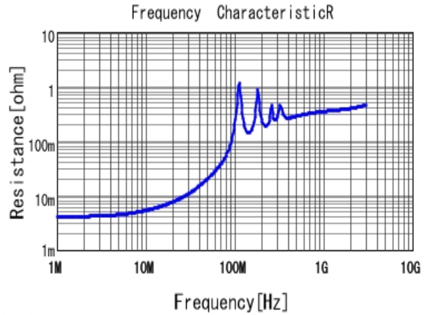
■ GRM32D7U2J103JW31 R DCOV, 25degC
