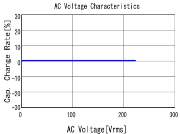
■ GRM32D7U2J103JW31 C-AC Voltage capchange, DCOV, 25.0d
