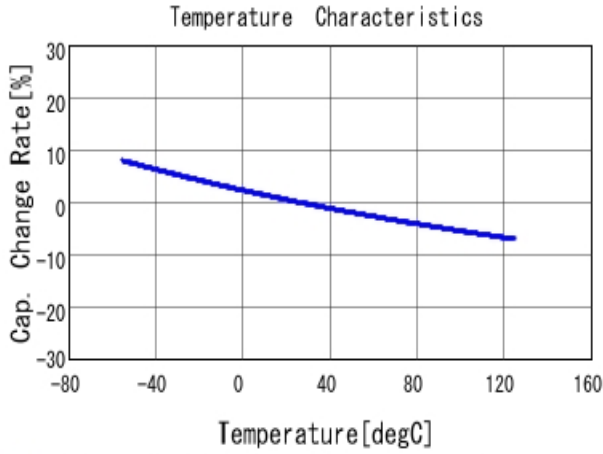
■ GRM32D7U2J103JW31 C-Temp. capchange, DCOV, AC1Vrms
