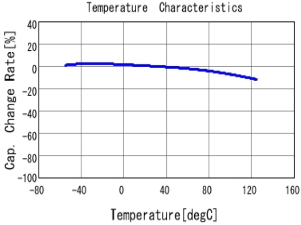
■ GRM31MR72A684KA35 C-Temp. capchange, DC0.0V, AC1.0V rm
