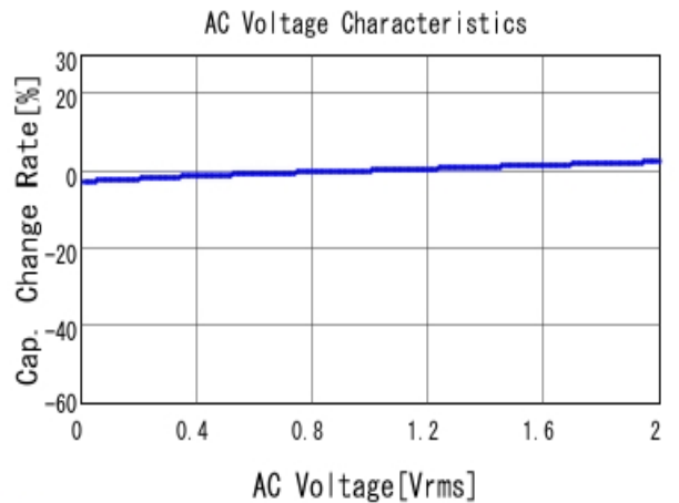
■ GRM31MR72A684KA35 C-AC Voltage capchange, DCOV, 25.0d
