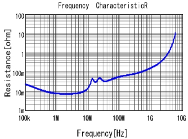
■ GRM31MR72A684KA35 R DCOV, 25degC
