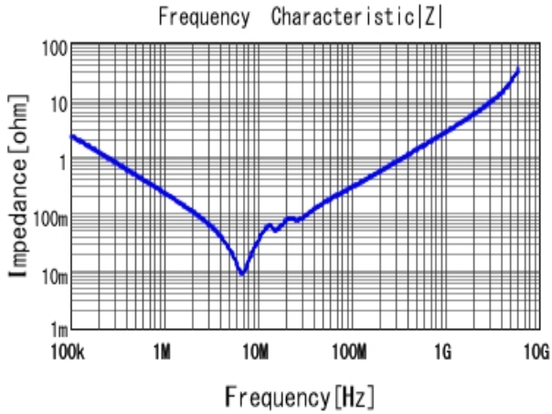
■ GRM31MR72A684KA35 |Z| DCOV, 25degC
