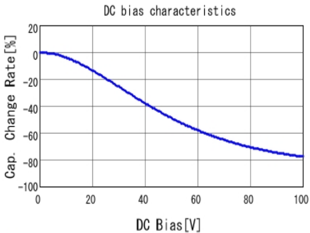
■ GRM31MR72A684KA35 C-DC bias capchange, 25.0degC, AC1.
