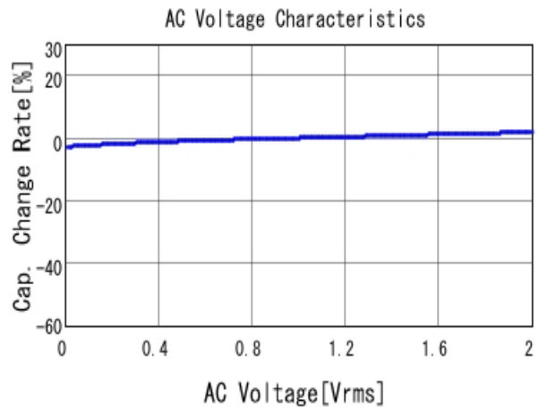
■ GRM31MR72A683KA01 C-AC Voltage capchange, DCOV, 25.0d
